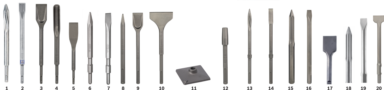
SDS-Plus shank (1 to 7)
